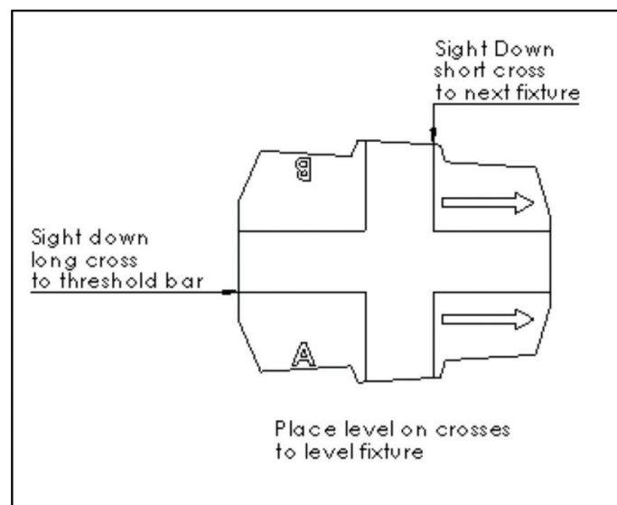
Figure 4: Fixture Aiming
